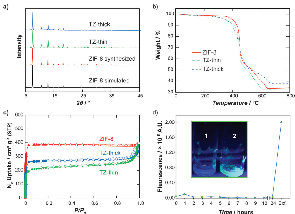
Figure 2. a) PXRD of simulated ZIF-8, synthesized ZIF-8, TZ-thin, and TZ-thick. b) TGA curves of ZIF-8, TZ-thin, and TZ-thick obtained in air atmosphere. c) \text{N}_2 sorption isotherm of ZIF-8, TZ-thin, and TZ-thick. The calculated BET surface area of ZIF-8, TZ-thick, and TZ-thin is 1537, 1053, and 847 \text{ m}^2 \text{g}^{-1} , respectively. d) Fluorescence measurement of the solution after centrifugation at each time point and after exfoliation of ZIF-8 (Exf.); inset: 1) growth solution and 2) fTMV@ZIF-8 under UV light.
